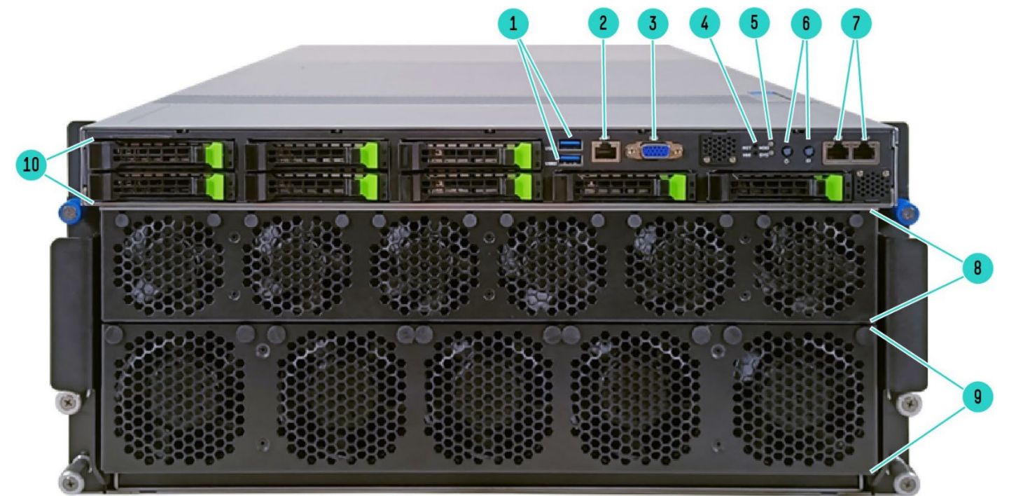
HPE Cray XD670 Server Front View
